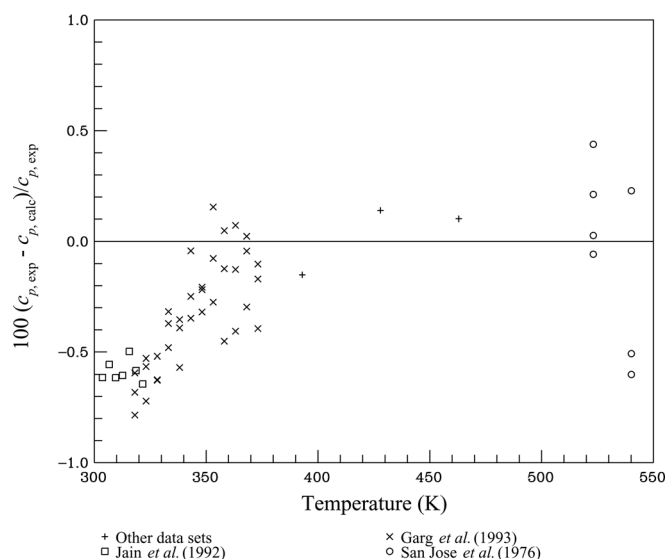
FIG. 14. Comparisons of isobaric heat capacities calculated with the equation of state to experimental data for m -xylene.
