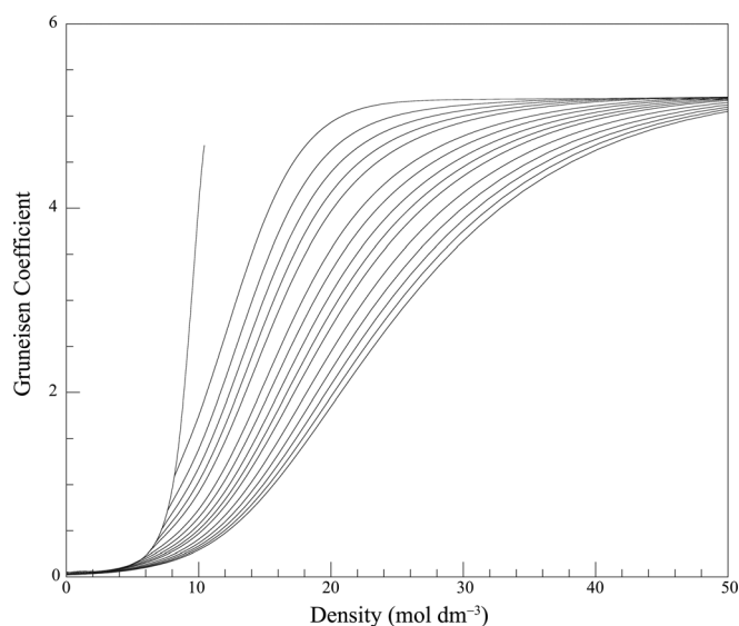
FIG. 31. Gruneisen coefficient versus density diagram plotted with the equation of state of p -xylene. Isotherms are shown at temperatures of ( T_{ip} , 350, 400, 450, 500, T_c , 700, 800, 900, 1000, 1200, 1400, 1600, 1800, and 2000) K.
