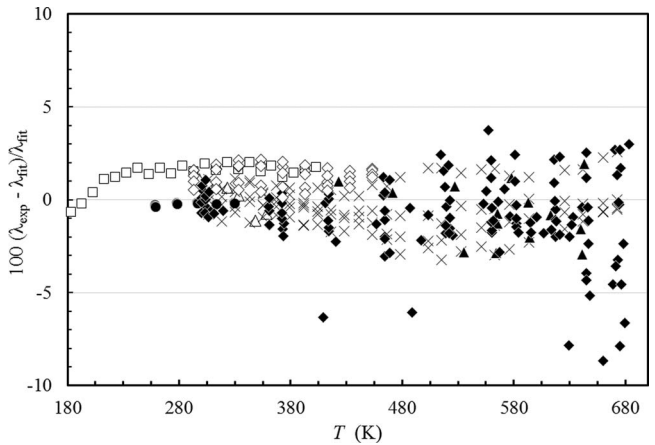
FIG. 30. Percentage deviations of primary experimental data of ethylbenzene from the values calculated by the present model, Eqs. (1), (6)–(10), and (18), as a function of temperature. Watanabe and Kato 27 (●), Kashiwagi et al. 29 (Δ), Mustafaev and Gabulov 30 (×), Rastorguev and Pugash 31 (◇), Kostrovski and Prostov 46 (▲), Akhundov 56 (◆), Brykov 57 (□).
