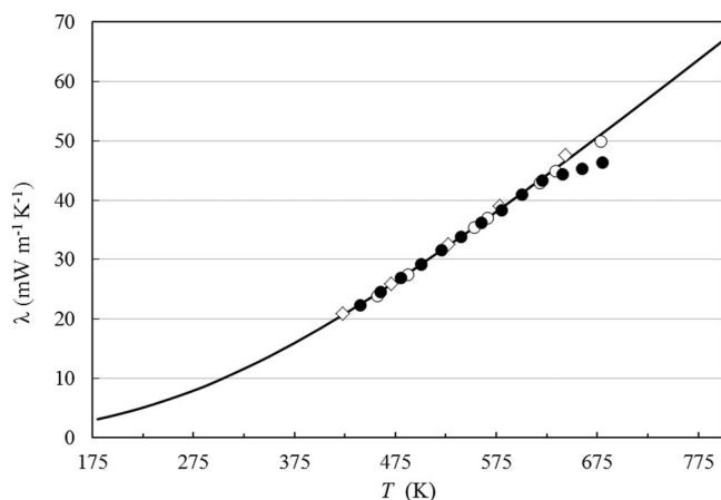
FIG. 27. Dilute-gas thermal conductivity of ethylbenzene as a function of temperature. Yaws 42 (---), Vargaftik 43 (●), Kostrovskii and Probstov 46 (◊), Akhundov 56 (○), Eq. (18) (—).
