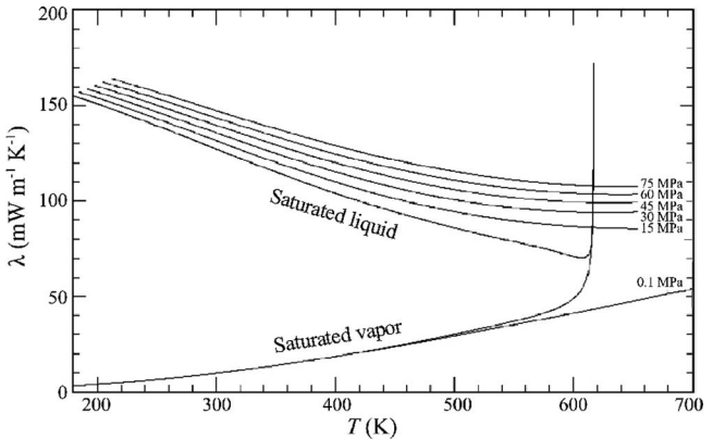
FIG. 32. Thermal conductivity of ethylbenzene as a function of temperature for different pressures.
