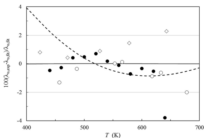
FIG. 28. Percentage deviations of the dilute-gas thermal conductivity of ethylbenzene from the scheme of Eqs. (3)–(5) and (17). Yaws 42 (---), Vargaftik 43 (●), Kostrovskii and Probstov 46 (◊), Akhundov 56 (○), Eq. (18) (—).
