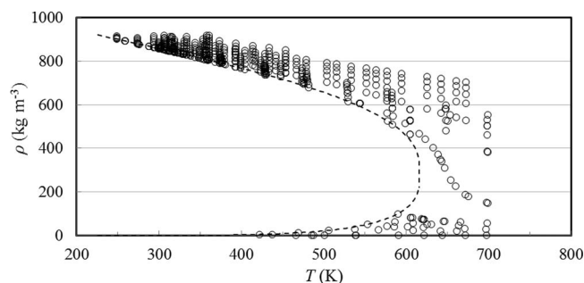
FIG. 10. Temperature-density ranges of the primary experimental thermal conductivity data for m -xylene. (–) saturation line.
