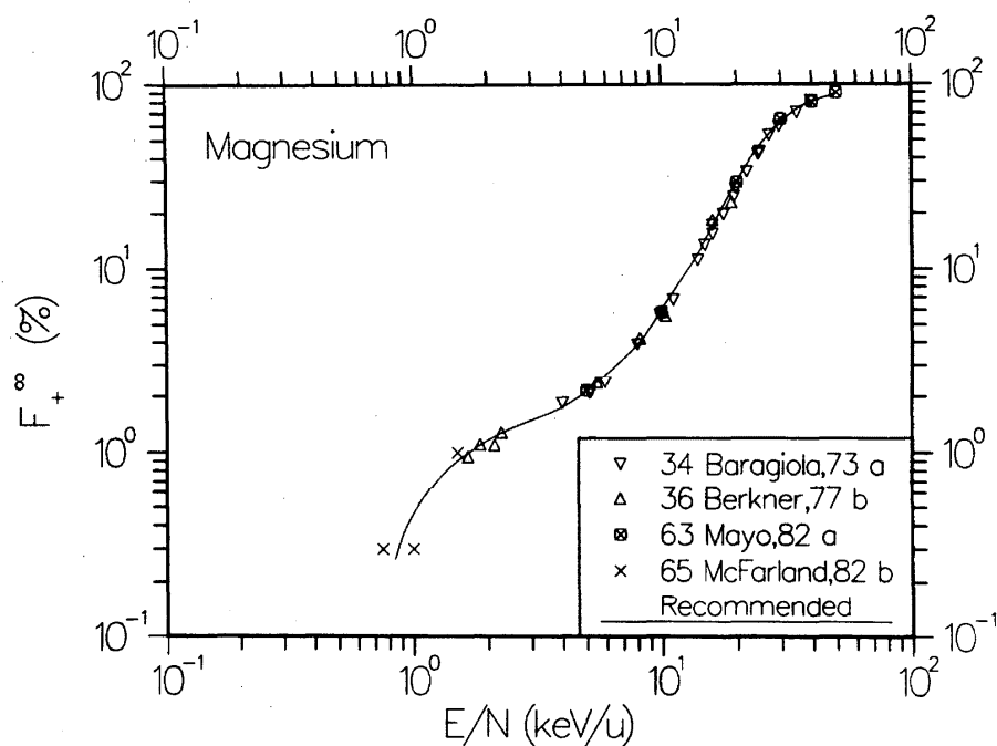
FIG. 56. Equilibrium fraction F_+^0 for hydrogen atoms and ions incident on Mg vapor.
