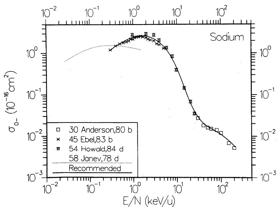
FIG. 15. Cross section \sigma_{0-} for electron capture in collisions of \text{H}^0 with Na vapor.
