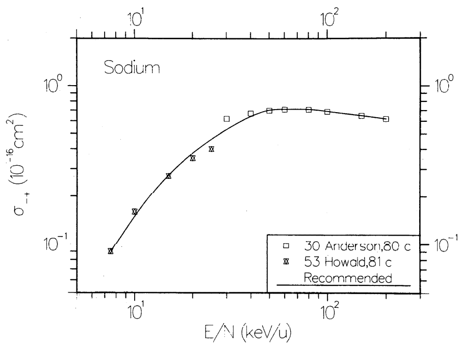
FIG. 16. Cross section \sigma_{+} for double electron loss in collisions of \text{H}^- with Na vapor.
