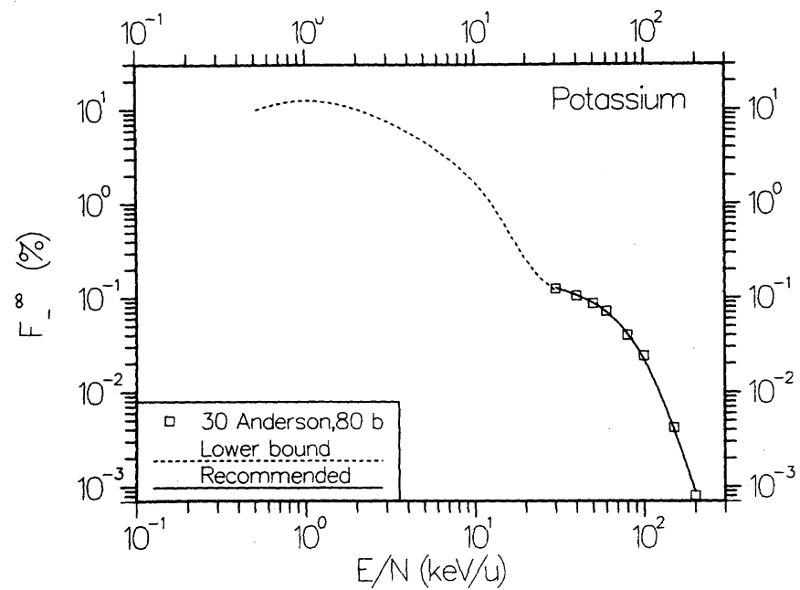
FIG. 30. Equilibrium fraction F_\infty^\infty for hydrogen atoms and ions incident on K vapor. The lower bound is based on data taken from Refs. 39, 50, and 86.
