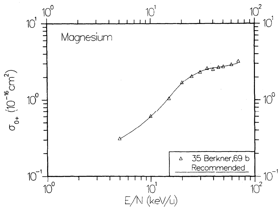
FIG. 54. Cross section \sigma_{0+} for electron loss in collisions of \text{H}^0 with Mg vapor.
