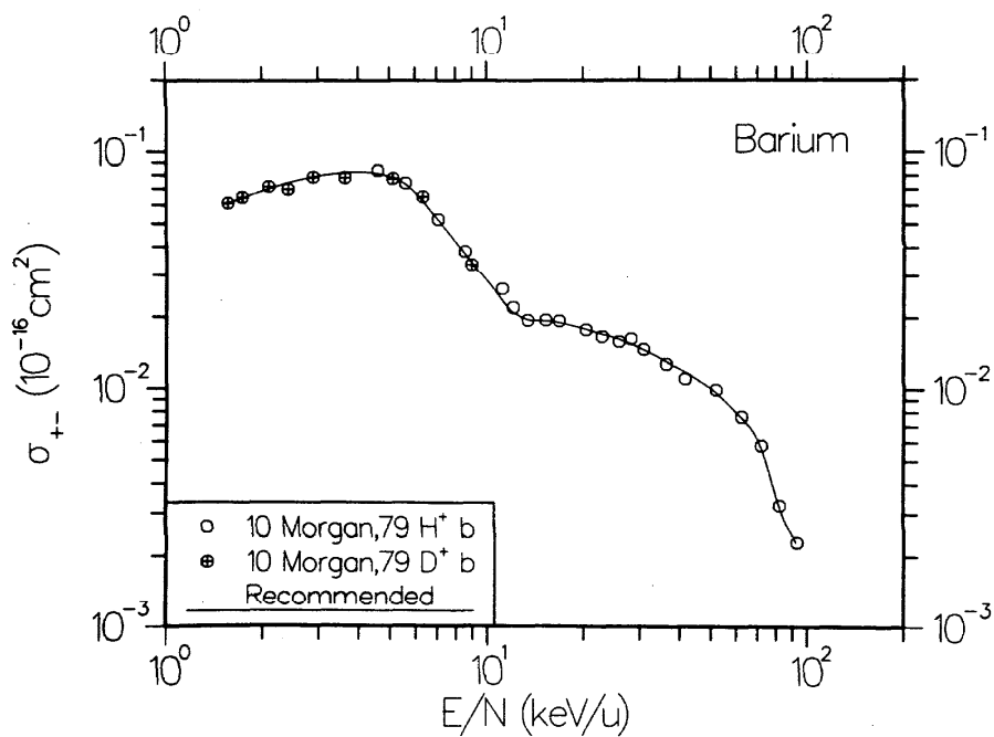
FIG. 72. Cross section \sigma_{+-} for double electron capture in collisions of \text{H}^+ with Ba vapor.
