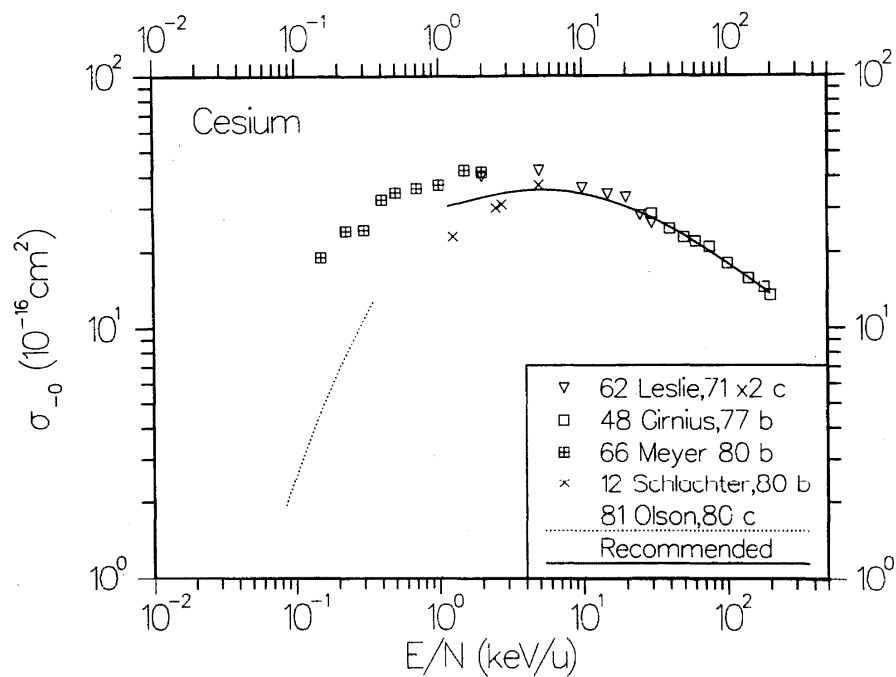
FIG. 47. Cross section \sigma_{-0} for detachment of electrons from \text{H}^- in collisions with Cs vapor.
