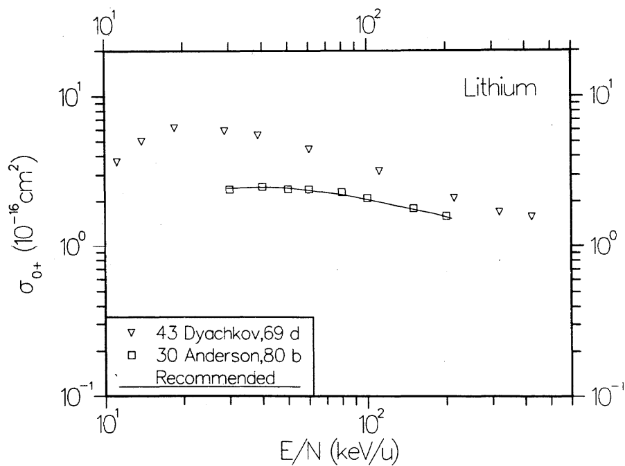
FIG. 4. Cross section \sigma_{0+} for electron loss in collisions of \text{H}^0 with Li vapor.
