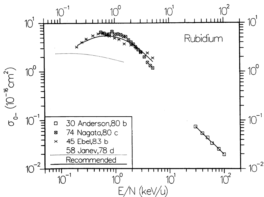
FIG. 35. Cross section \sigma_{0-} for electron capture in collision of \text{H}^0 with Rb vapor.
