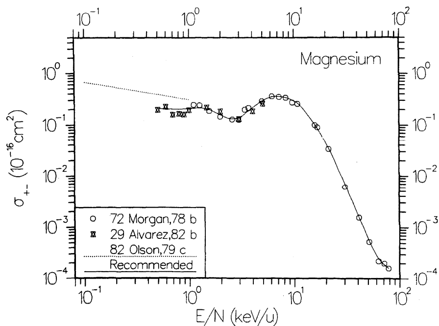
FIG. 53. Cross section \sigma_{+-} for double electron capture in collisions of \text{H}^+ with Mg vapor.
