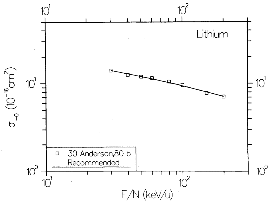
FIG. 7. Cross section \sigma_{-0} for detachment of electrons from \text{H}^- in collisions with Li vapor.
