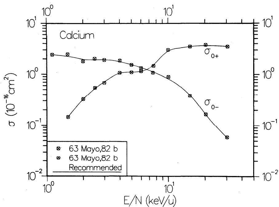
FIG. 60. Cross sections \sigma_{0+} for electron loss and \sigma_{0-} for electron capture in collisions of H^0 with Ca vapor.
