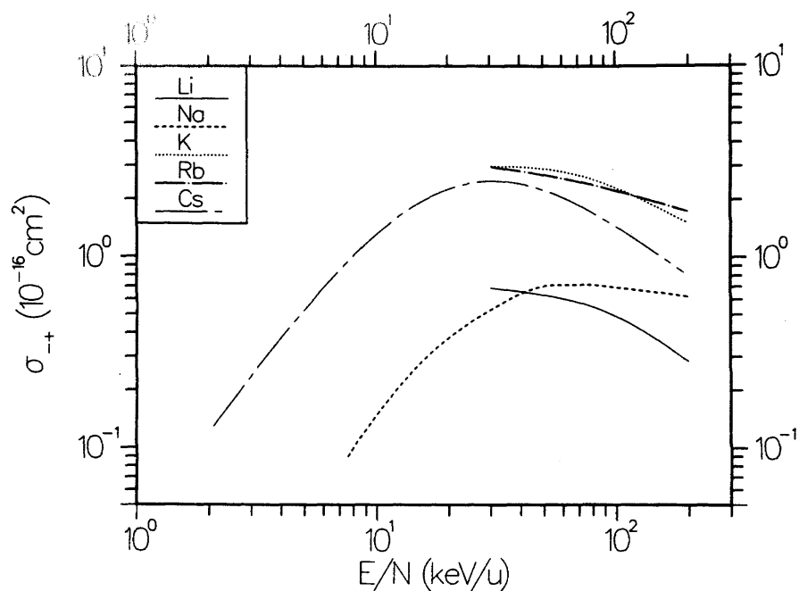
FIG. 93. Recommended values for \sigma_{-+} , the cross section for double electron loss, in collisions of H^- ions with alkali metal vapors.
