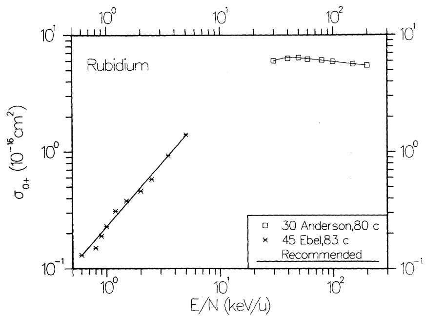
FIG. 34. Cross section \sigma_{0+} for electron loss in collisions of \text{H}^0 with Rb vapor.
