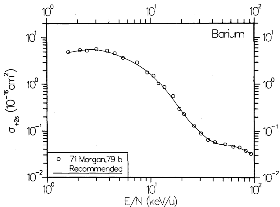
FIG. 71. Cross section \sigma_{+2s} for electron capture into the 2s state of the neutral hydrogen atom in collisions of \text{H}^+ with Ba vapor.
