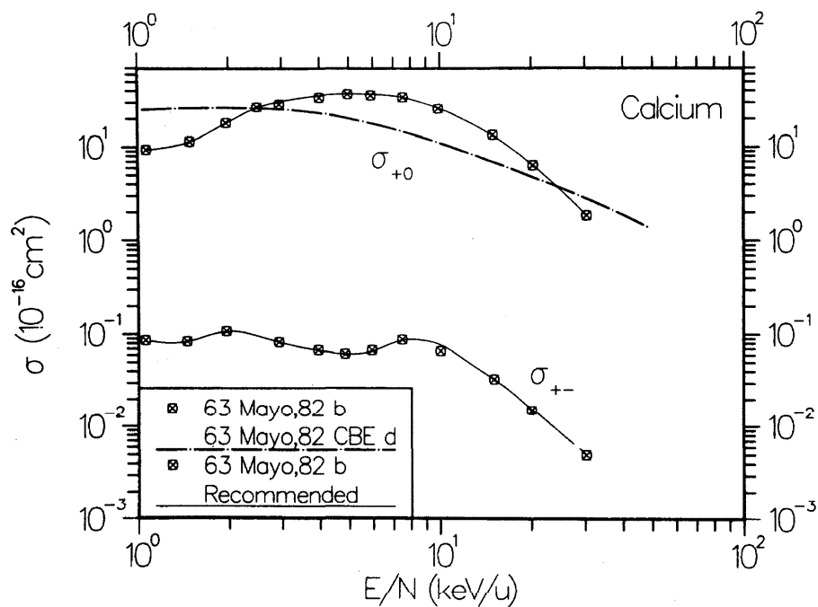
FIG. 59. Cross sections \sigma_{+0} for single electron capture and \sigma_{+-} for double electron capture in collisions of H^+ with Ca vapor.
