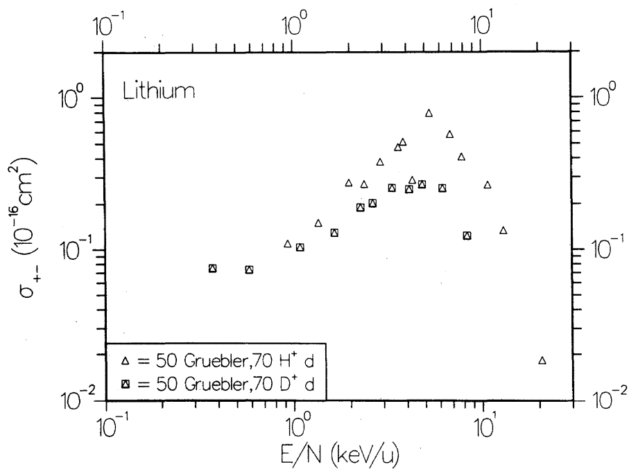
FIG. 3. Cross section \sigma_{+-} for double electron capture in collisions of \text{H}^+ with Li vapor.
