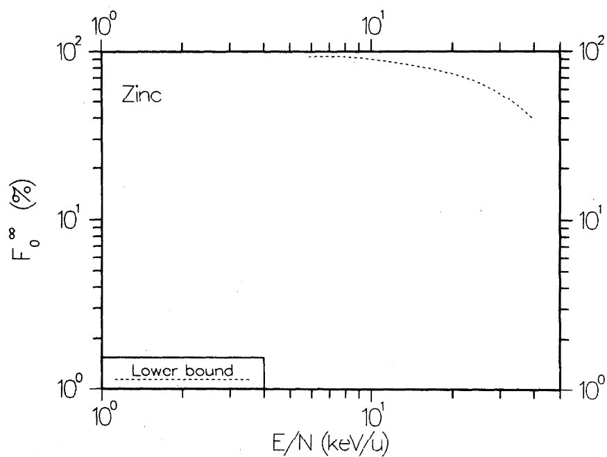
FIG. 76. Equilibrium fraction F_0 for hydrogen atoms and ions incident on Zn vapor. The lower bound is based on data taken from Ref. 44.
