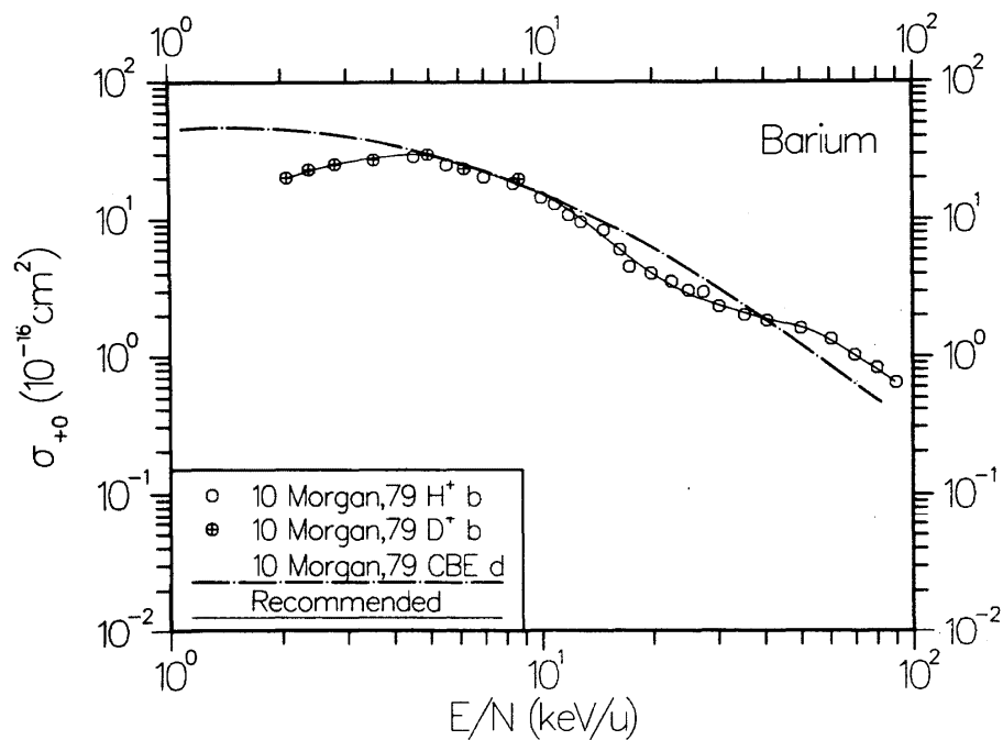
FIG. 70. Cross section \sigma_{+0} for electron capture into all states of the neutral hydrogen atom in collisions of \text{H}^+ with Ba vapor.
