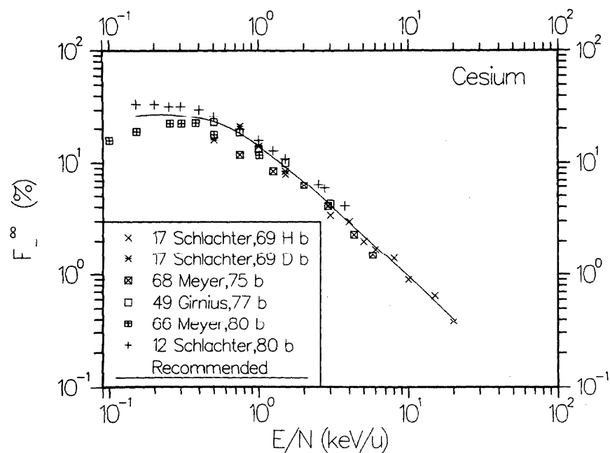
FIG. 50. Equilibrium fraction F_1^\infty for hydrogen atoms and ions incident on Cs vapor.
