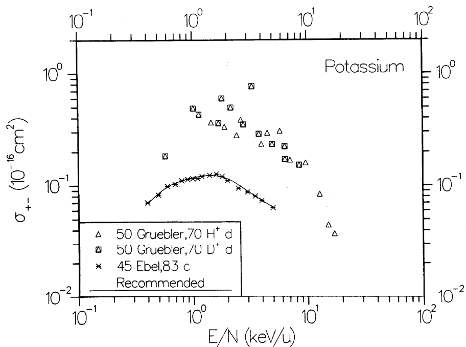
FIG. 23. Cross section \sigma_{+-} for double electron capture in collisions of \text{H}^+ with K vapor.
