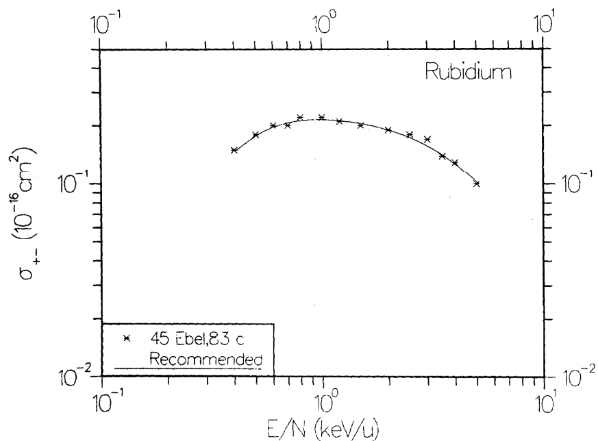
FIG. 33. Cross section \sigma_{+-} for double electron capture in collisions of \text{H}^+ with Rb vapor.
