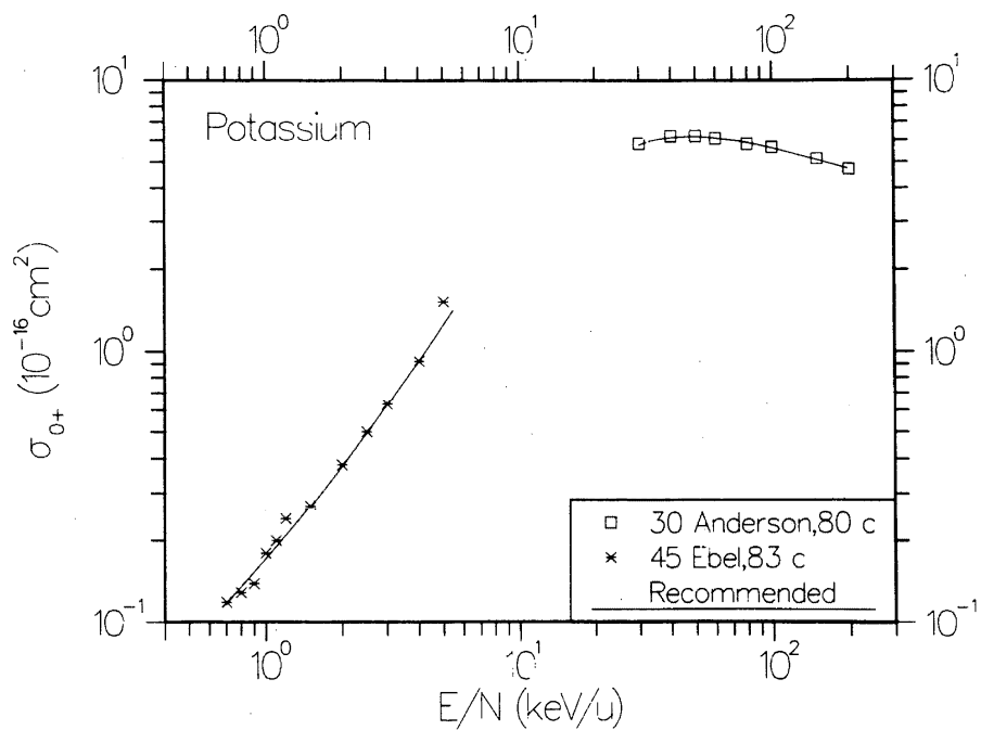
FIG. 24. Cross section \sigma_{0+} for electron loss in collisions of \text{H}^0 with K vapor.
