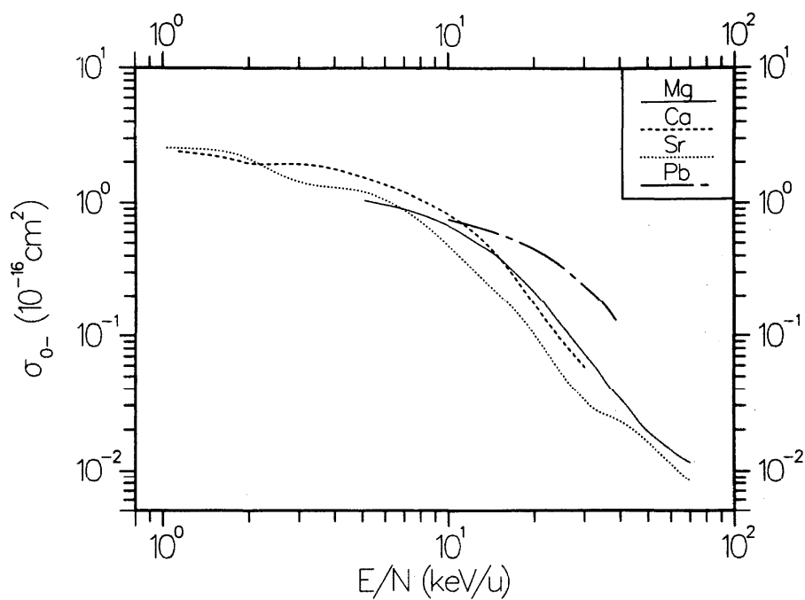
FIG. 90. Recommended values for \sigma_{0-} , the cross section for electron capture, in collisions of H^0 with alkaline-earth and lead vapors.
