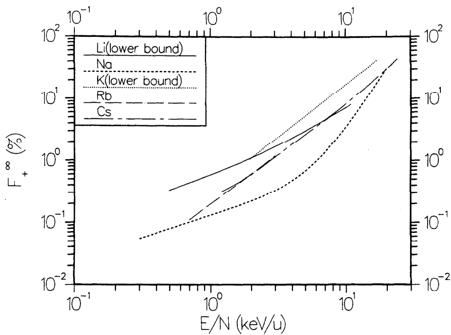
FIG. 94. Recommended values for F_{+}^{\infty} , the equilibrium fraction for formation of H^+ ions, in collisions of hydrogen atoms and ions with alkali metal vapors.
