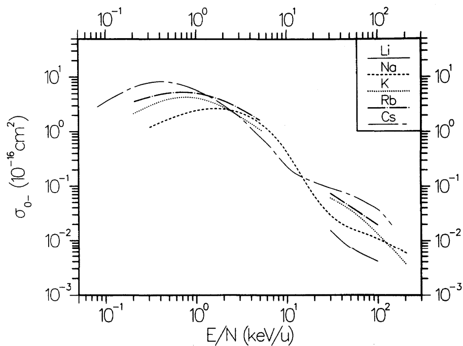
FIG. 89. Recommended values for \sigma_{0-} , the cross section for electron capture, in collisions of H^0 with alkali metal vapors.
