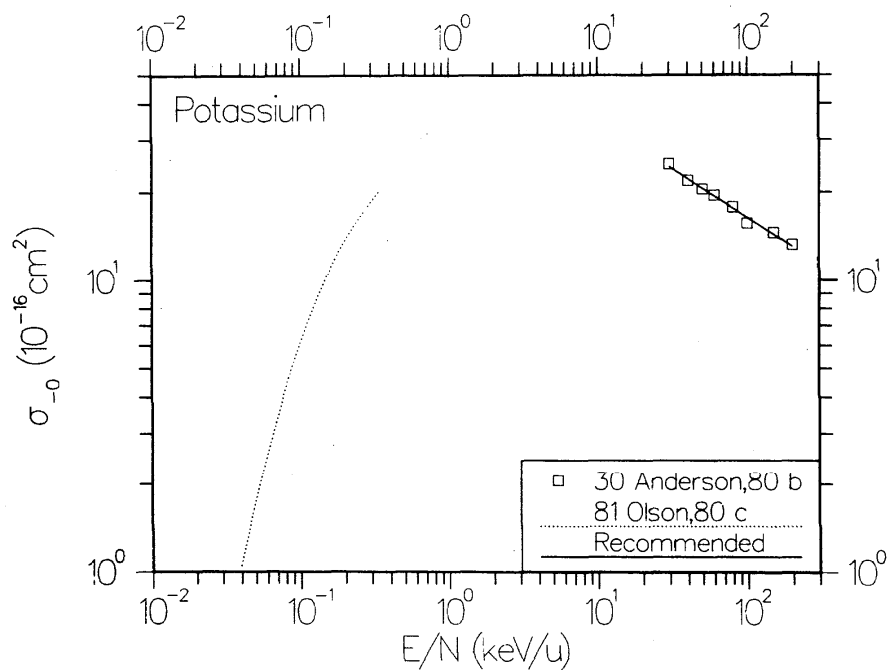
FIG. 27. Cross section \sigma_{-0} for detachment of electrons from \text{H}^- in collisions with K vapor.
