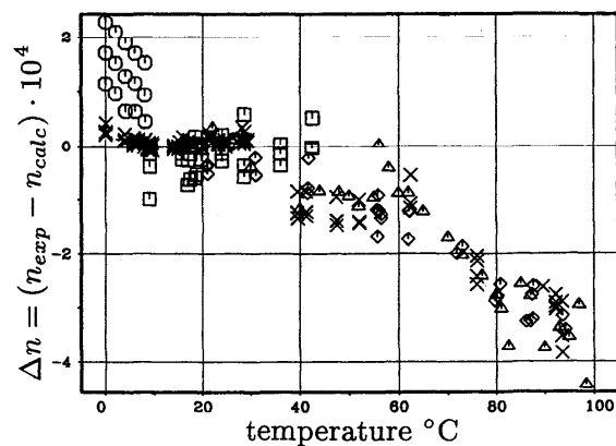
FIG. 16. Departures from the formulation of medium- and high-quality n data in the visible and in the temperature range of 0 to 100 °C. The data are by Bender 57 , Damien 54 , Hall 23 , Hawkes 35 , Jasse 24 and Ketteler 58 .
