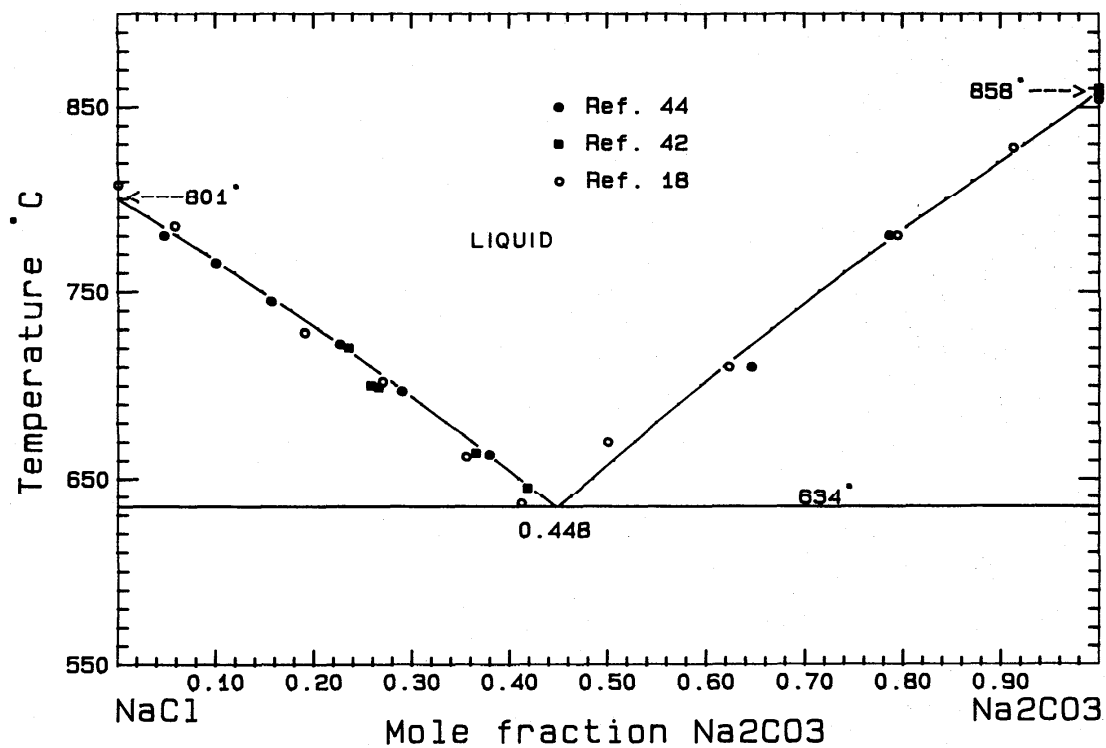
FIG. 8. The system \text{NaCl-Na}_2\text{CO}_3 .
