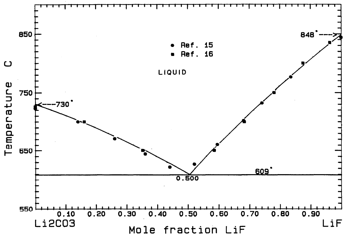
FIG. 1. The system \text{Li}_2\text{CO}_3 - \text{LiF} .
