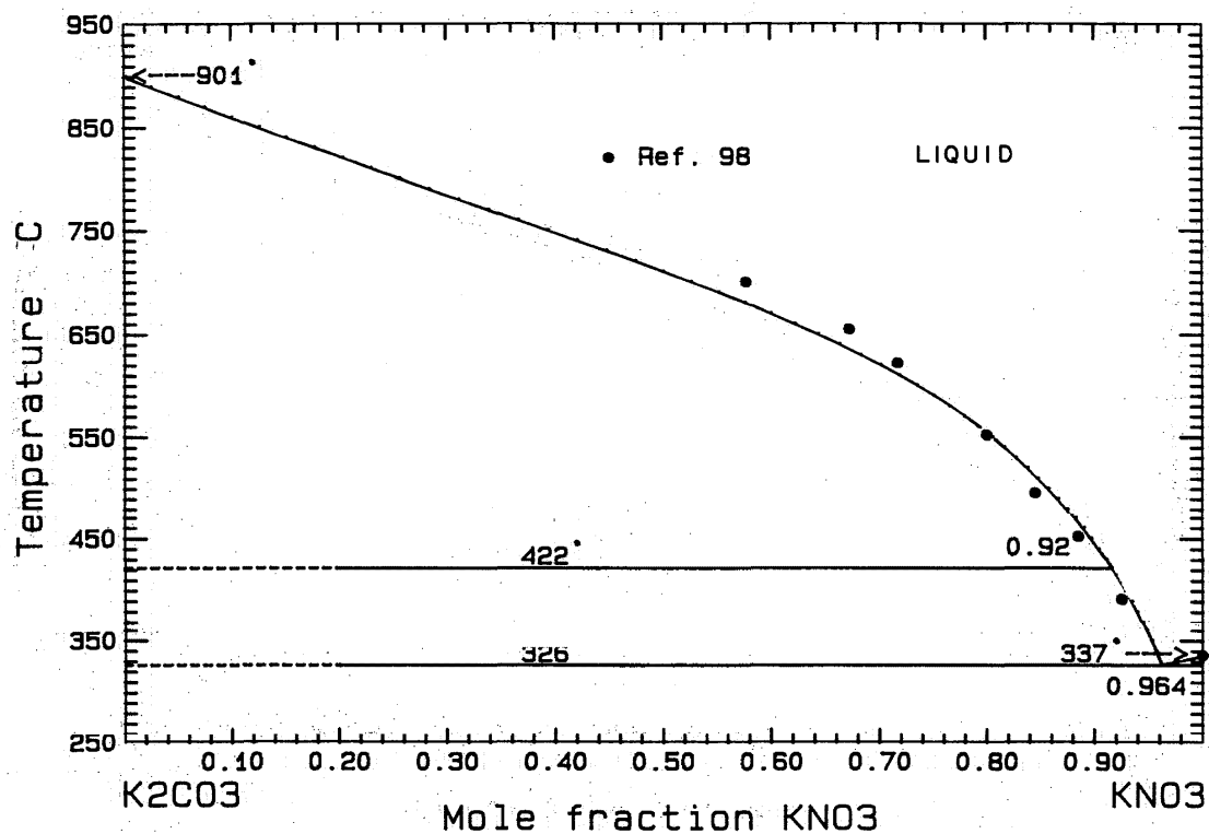
FIG. 25. The system \text{K}_2\text{CO}_3 - \text{KNO}_3 .
