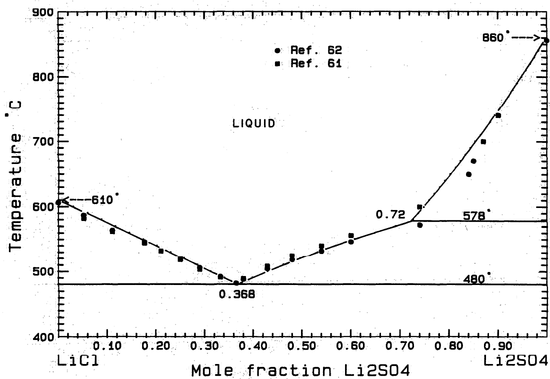
FIG. 10. The system LiCl-Li 2 SO 4 .
