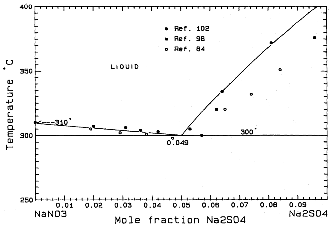
FIG. 28. The system \text{NaNO}_3 - \text{Na}_2\text{SO}_4 enlarged.
