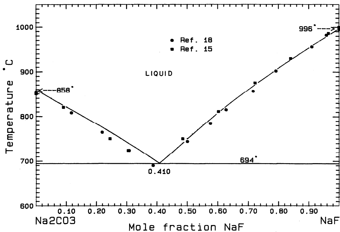
FIG. 2. The system \text{Na}_2\text{CO}_3 - \text{NaF} .
