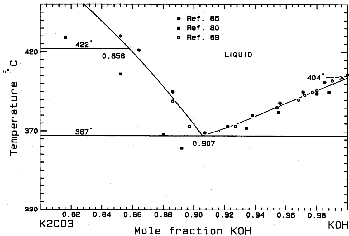
FIG. 17. The system \text{K}_2\text{CO}_3 - \text{KOH} enlarged.
