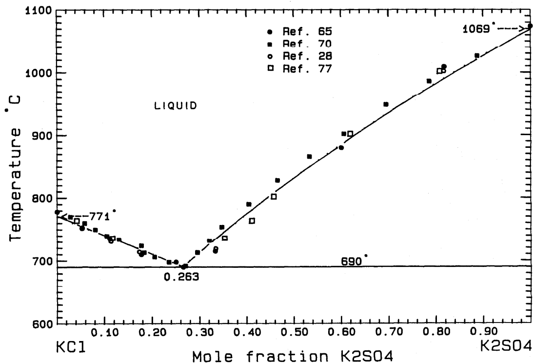
FIG. 12. The system KCl-K 2 SO 4 .
