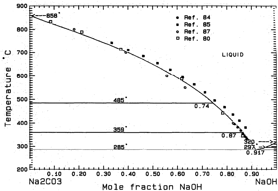
FIG. 14. The system \text{Na}_2\text{CO}_3 - \text{NaOH} .
