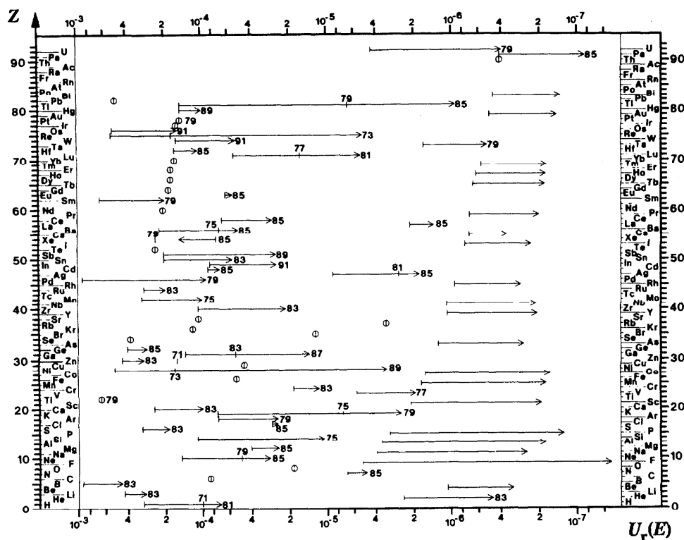
Fig. 1. Changes in U_r(E) from 1969 to 1991 (Ref. 22). The symbol \odot indicates no change. Number where given is last two digits of the year of the last change. Number (year) is not listed for monoisotopic elements. Intermediate changes for all but the monoisotopic elements are indicated by short vertical lines together with the year of the change.
