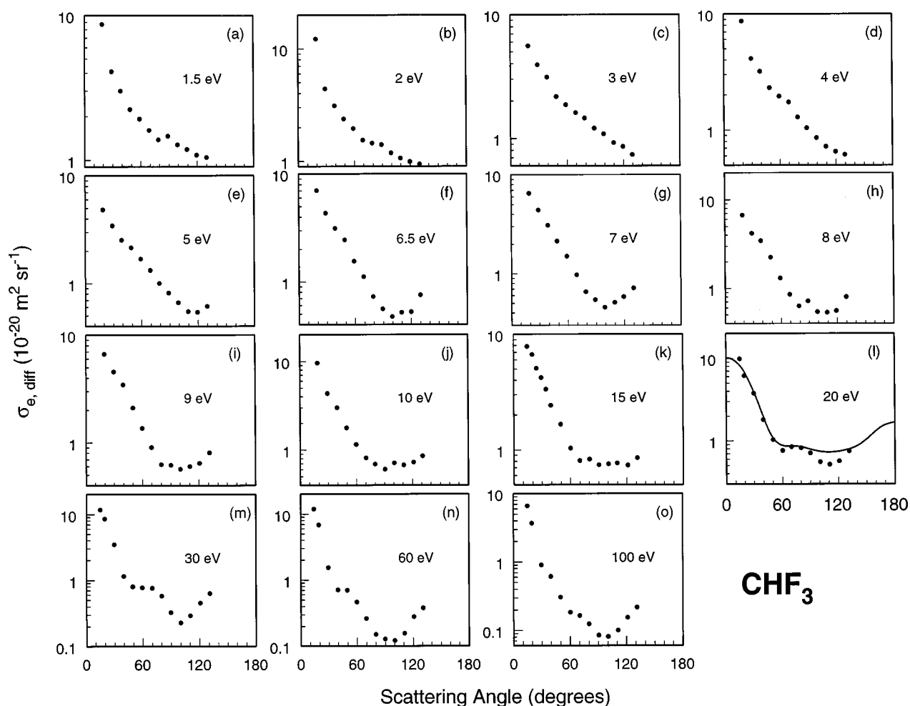
Fig. 9. Measured elastic differential electron scattering cross sections \sigma_{e,\text{diff}}(\varepsilon) , for CHF 3 from Refs. 58 and 59. A recent calculated result from Ref. 60 is also shown (—) for 20 eV.
