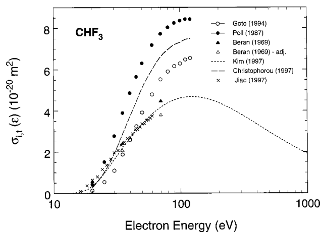
FIG. 12. Total ionization cross sections, \sigma_{i,t}(\varepsilon) , for \text{CHF}_3 as obtained by summing up the partial ionization cross sections, \sigma_{i,\text{part}}(\varepsilon) : (●) Ref. 63; (○) Ref. 64; (×) recent data from Ref. 61. Also shown are the data of Ref. 65 (▲), the adjusted data of Ref. 65 (△), the calculated values from Ref. 34 (---), and the previously suggested values from Ref. 2 (—).
