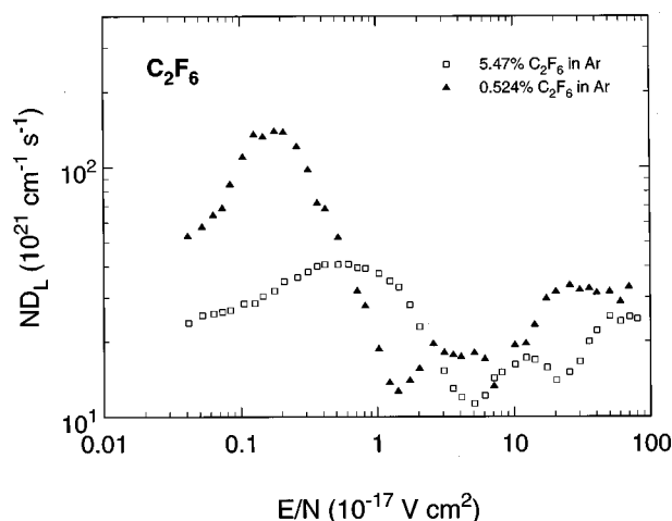
FIG. 16. Measurements of the product of the gas density and longitudinal electron diffusion coefficient, ND_L(E/N) , for 5.47% C 2 F 6 in Ar (□) and 0.524% C 2 F 6 in Ar (▲) from Ref. 73.
