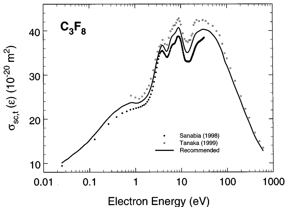
FIG. 17. Total electron scattering cross section, \sigma_{sc,t}(\epsilon) , for C 3 F 8 : (●) measurements of Ref. 56; (○) recent measurements of Ref. 74; (—) updated recommended values.
