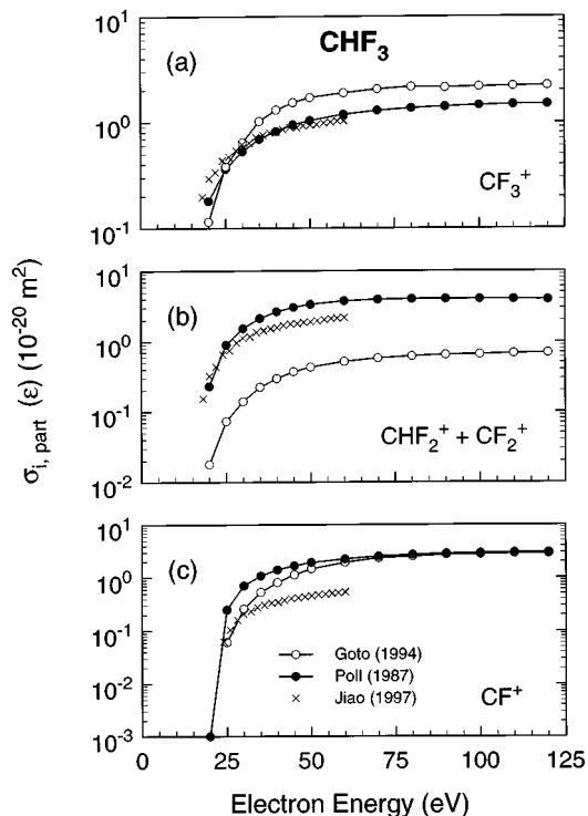
FIG. 11. Partial ionization cross sections, \sigma_{i,\text{part}}(\varepsilon) , for \text{CHF}_3 for the product ions indicated: (●) Ref. 63; (○) Ref. 64; (×) recent data of Ref. 61.
