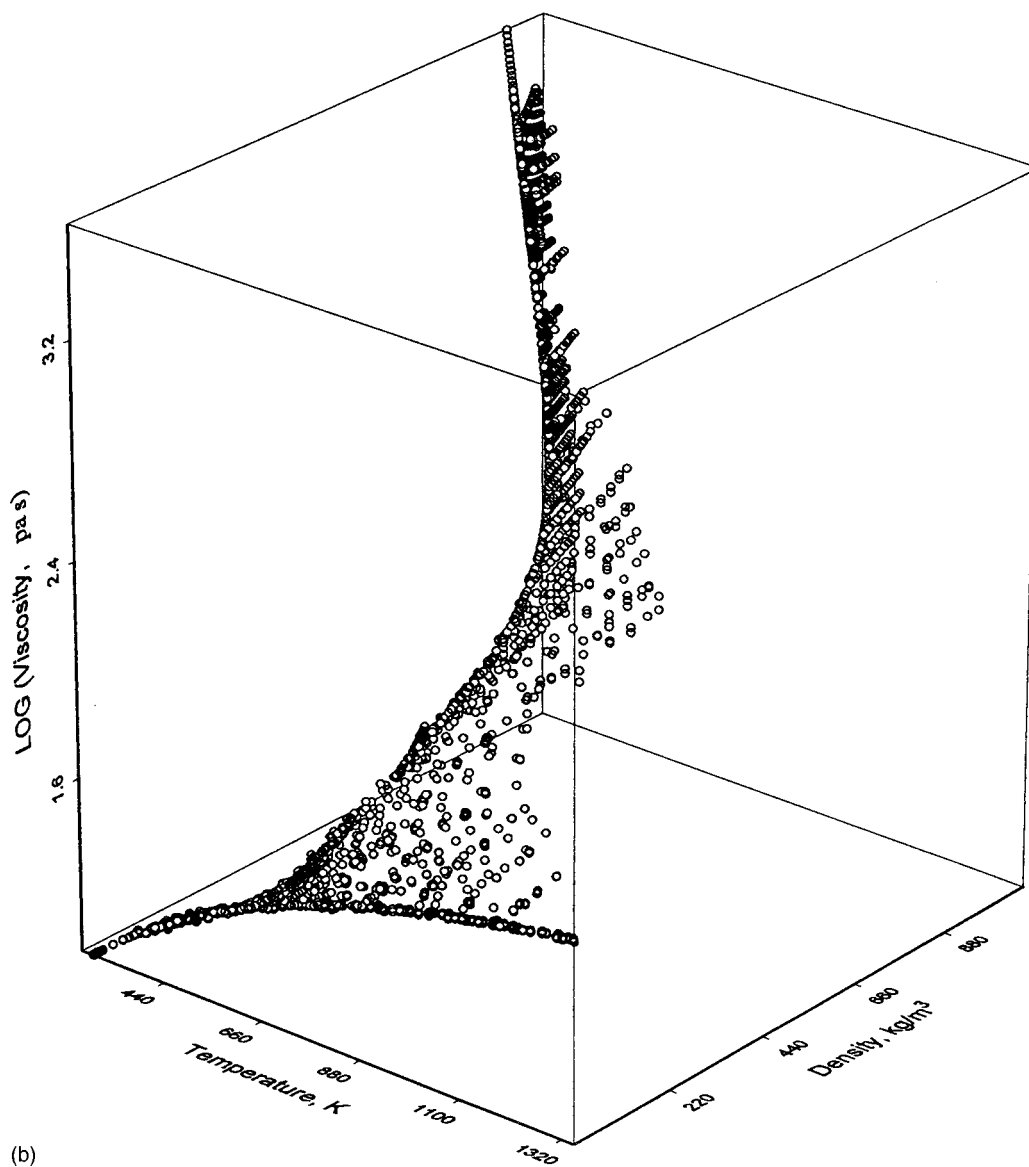
FIG. 1. (a) Temperature and pressure ranges of viscosity measurements considered; (b) Experimental viscosity as function of temperature and density; (c) Temperature and pressure ranges of thermal-conductivity measurements considered; (d) Experimental thermal conductivity as function of temperature and density.
