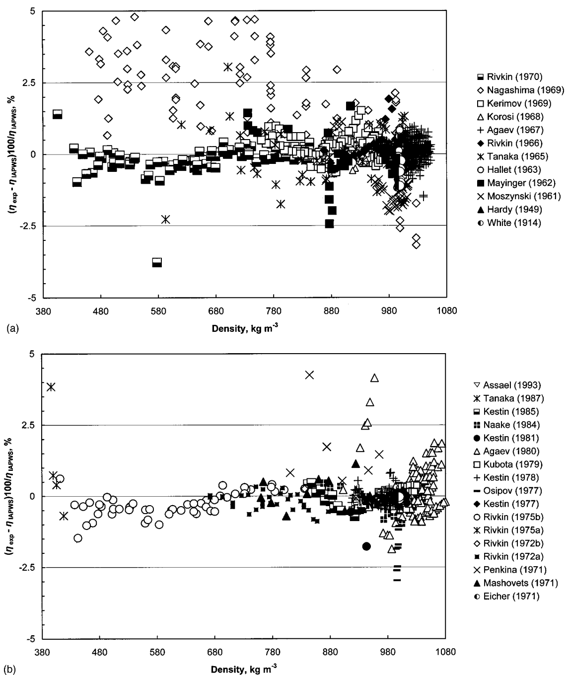
FIG. 3. (a) and (b) Deviations of viscosity measurements of water in the liquid phase (excluding data near 0.101 325 MPa) from the IAPWS correlation.
